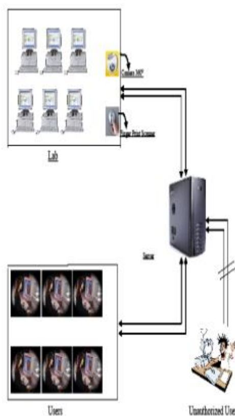
Figure1: System architecture
